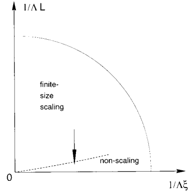
Fig. 1. Asymptotic L^{-1} - \xi^{-1} plane (schematic plot) above T_c for the \varphi^4 field-theoretic model at finite cutoff \Lambda in the large- n limit in three dimensions where L is the system size and \xi is the bulk correlation length. Finite-cutoff effects become non-negligible in the non-scaling region below the dotted line. This crossover line has a vanishing slope at the origin and is determined by equation (15) with \gamma/\nu = 2 , \gamma = 2 and a_1(3, 0) = 0.226 for d = 3 . Well above this line the cutoff dependence is negligible in equation (11). The arrow indicates an approach towards bulk critical behavior at constant 0 < t \ll 1 through the non-scaling region where equation (14) is valid.
